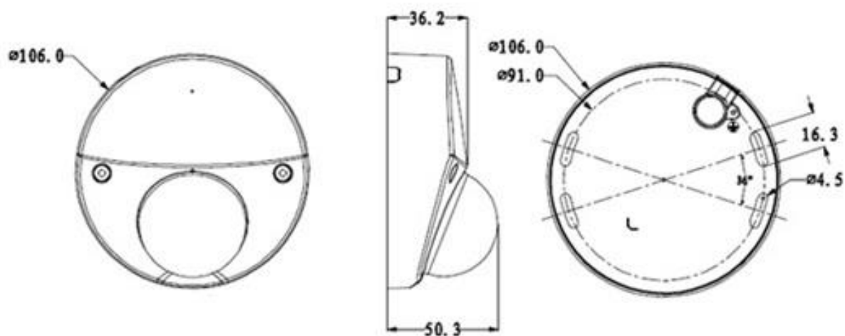
Figure 2-2 GEODOME – LE 339HD Dimensions
